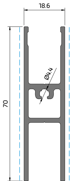
OR 42 Travessa Transom | Traverse
