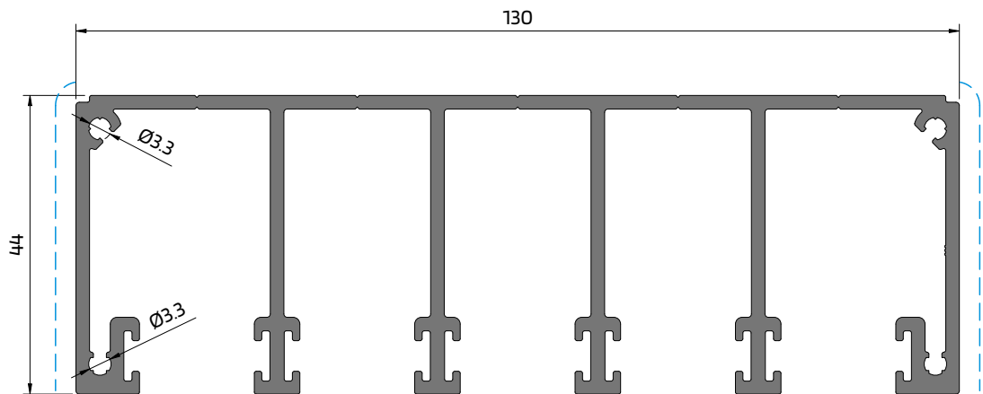
OR 40 Padeira 5-rail 5-rail Lintel | Linteau 5-rail
