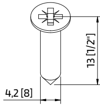
290061 PARAF. DIN7982 PH 4,2x13 INOX A2 SCREW VIS
