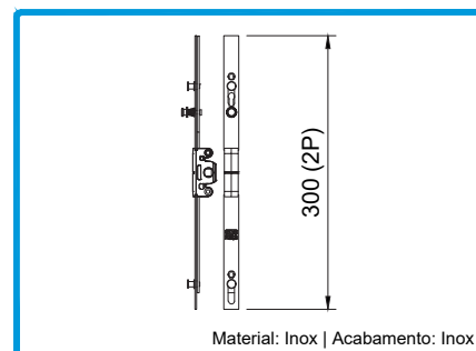
211119 F. MULTIP. ANTI-FALSA MAN. 300
