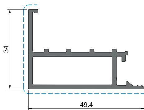
JT 51 Perfil central Central profile | Profilé central
