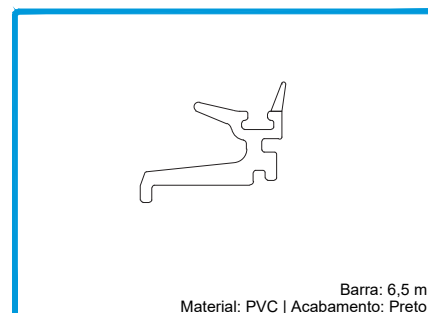
208351 JUNTA CENTRAL 2197 JT-SLIM
