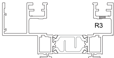
Rasgo | Hole | Rainure R3: 5x20mm
