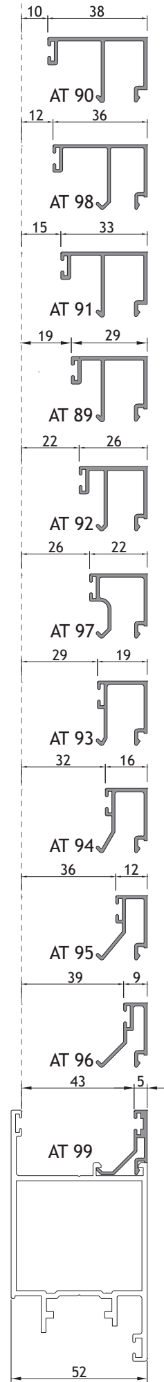
PERFIS DE 52mm PROFILES OF 52mm PROFILS DE 52mm
