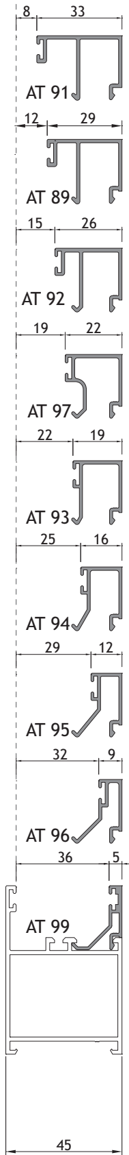
PERFIS DE 45mm PROFILES OF 45mm PROFILS DE 45mm
