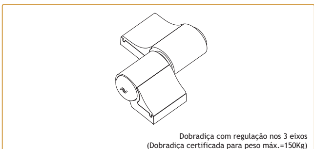
202010 DOBRADIÇA MECANICA 2 ABAS 1145/60 202012 DOBRADIÇA MECANICA 2 ABAS 1145/79 202020 DOBRADIÇA MECANICA 2 ABAS 1145/93SM
