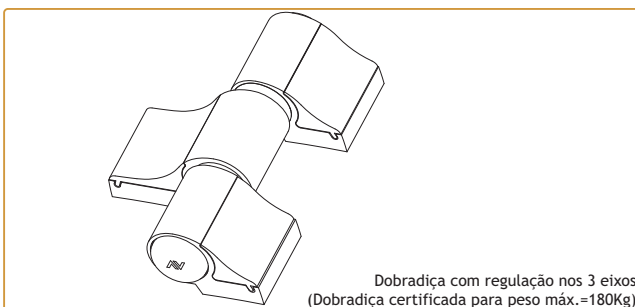
202610 DOBRADIÇA MECANICA 3 ABAS 1145.3/60
