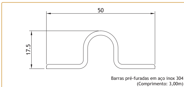
GUIA INOX PA 20049 (3m)
