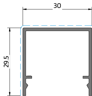
SQ 30 Capa 30x30 Cover | Capot
