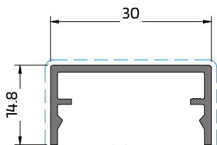
SQ 15 Capa 30x15 Cover | Capot
