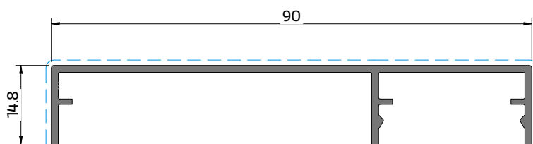
SQ 16 Capa 90x15 Cover | Capot
