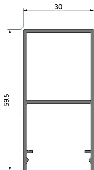
SQ 60 Capa 30x60 Cover | Capot
