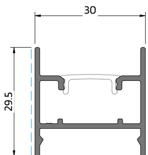
SQ 41 Capa 30x30 Hled Cover | Capot
