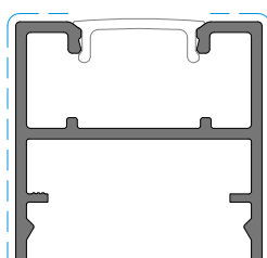
SQ 31 Capa 30x30 Qled Cover | Capot
